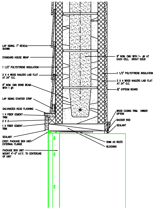
HEAD DETAIL
