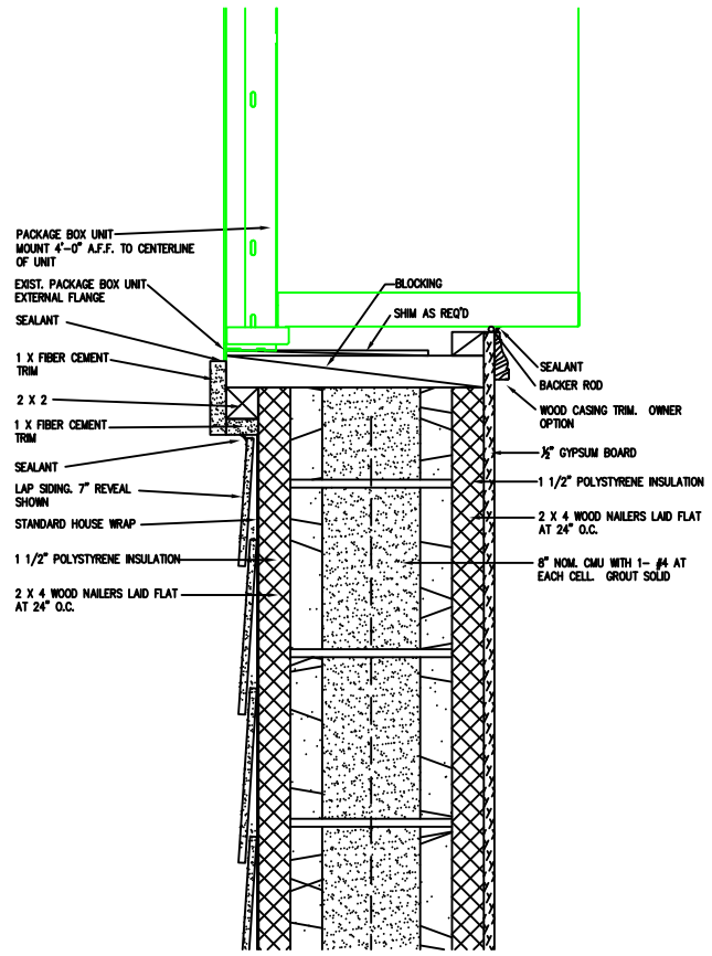
SILL DETAIL
